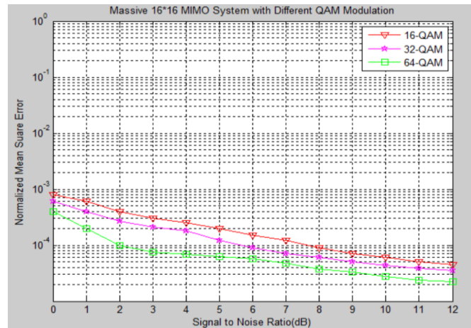
Figure 5: NMSE of Massive 16×16 System with Machine Learning based Channel Estimation Technique
